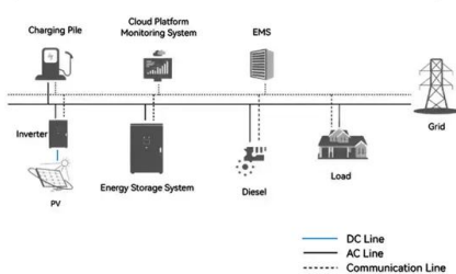
System Topology
